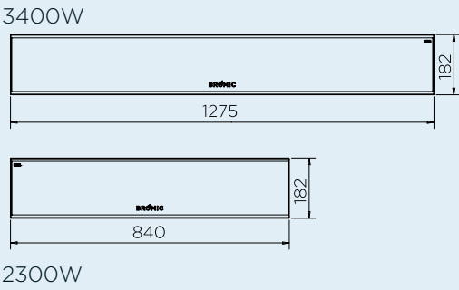
PRODUCT MEASUREMENTS
