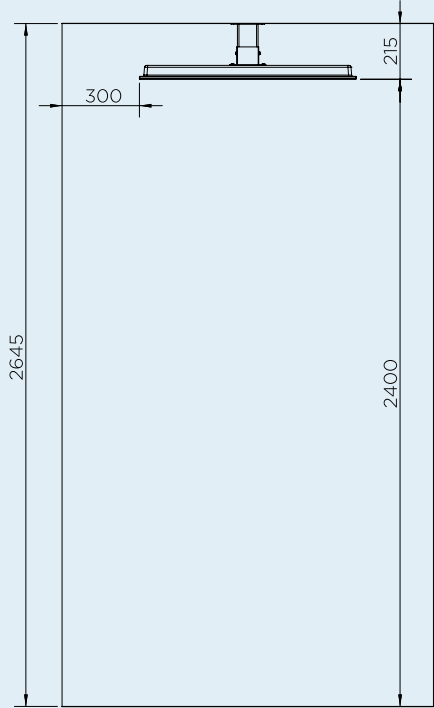
CEILING MOUNT CLEARANCE
