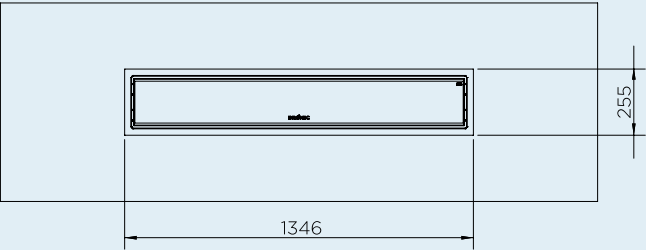
CEILING RECESS FRAME 3400W
