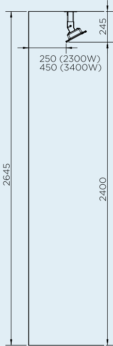
ANGLE MOUNT
