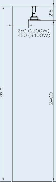
FRONT DOWN MOUNT
