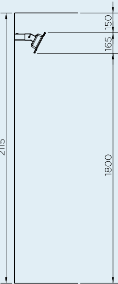
WALL MOUNT CLEARANCE
