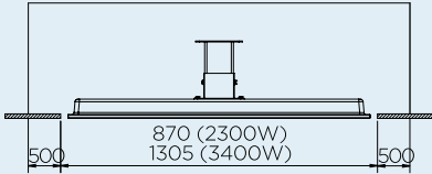
MINIMUM CAVITY OPTION 1
