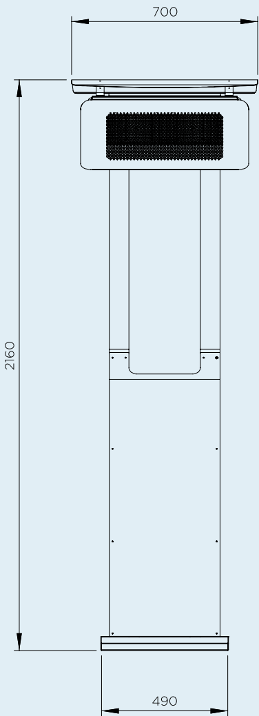
PRODUCT MEASUREMENTS
