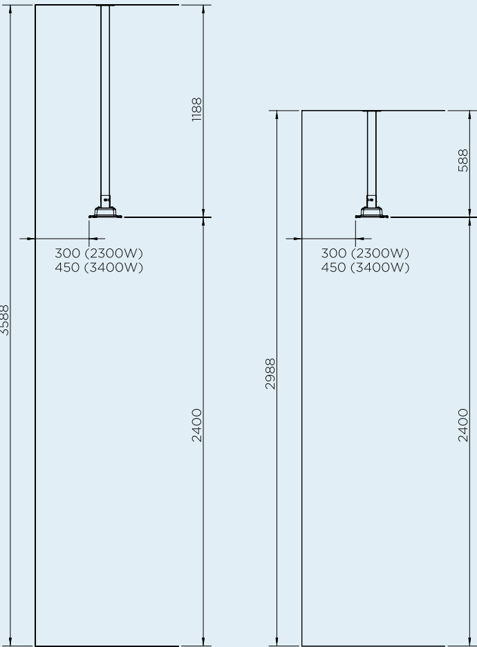
CEILING POLE CLEARANCE
