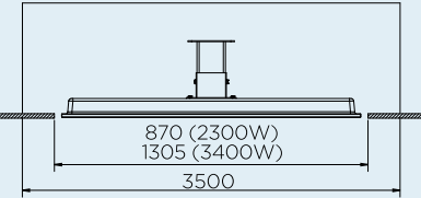
MINIMUM CAVITY OPTION 2
