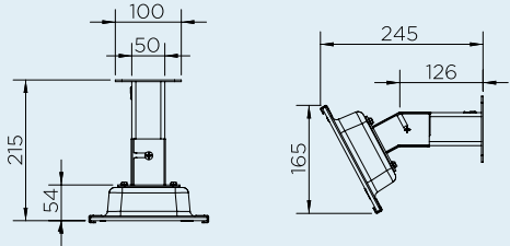
BRACKET MEASUREMENTS
